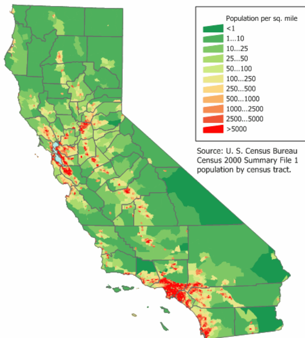
Figure 73: Population intensities 56
