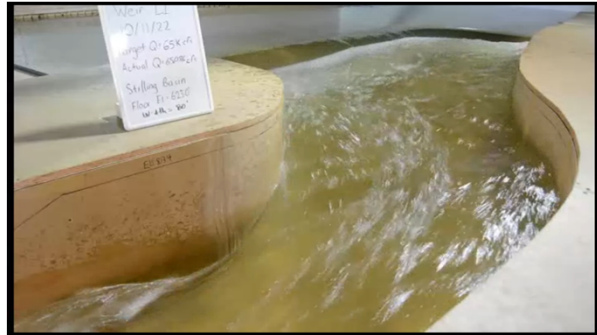
Santiago Creek Dam Spillway Physical Model
