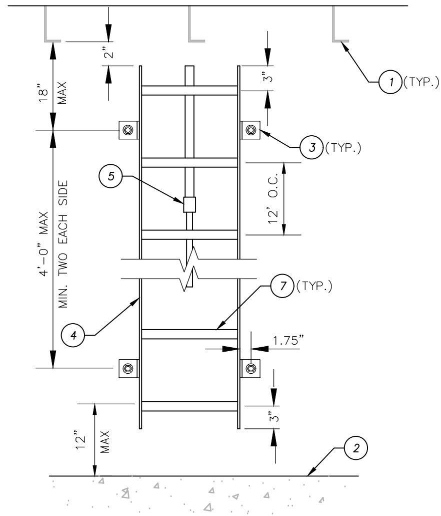
FRONT VIEW CENTER SAFETY POST OPTION
