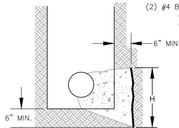
SECTION HORIZONTAL BEND
