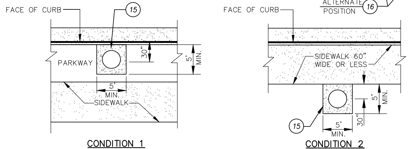
FLUSH-OUT ASSEMBLY LOCATION PLANS
