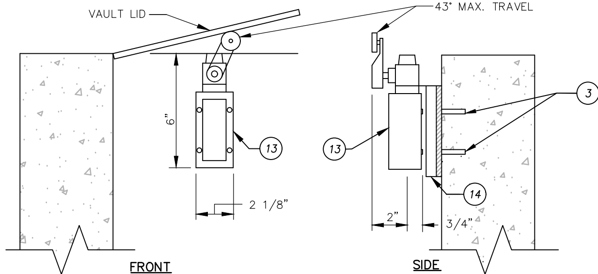
INTRUSION SWITCH
