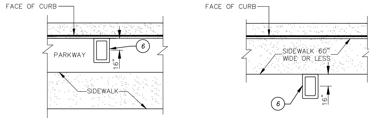
CONDITION 1 CONDITION 2 2" FLUSH-OUT ASSEMBLY LOCATION PLANS
