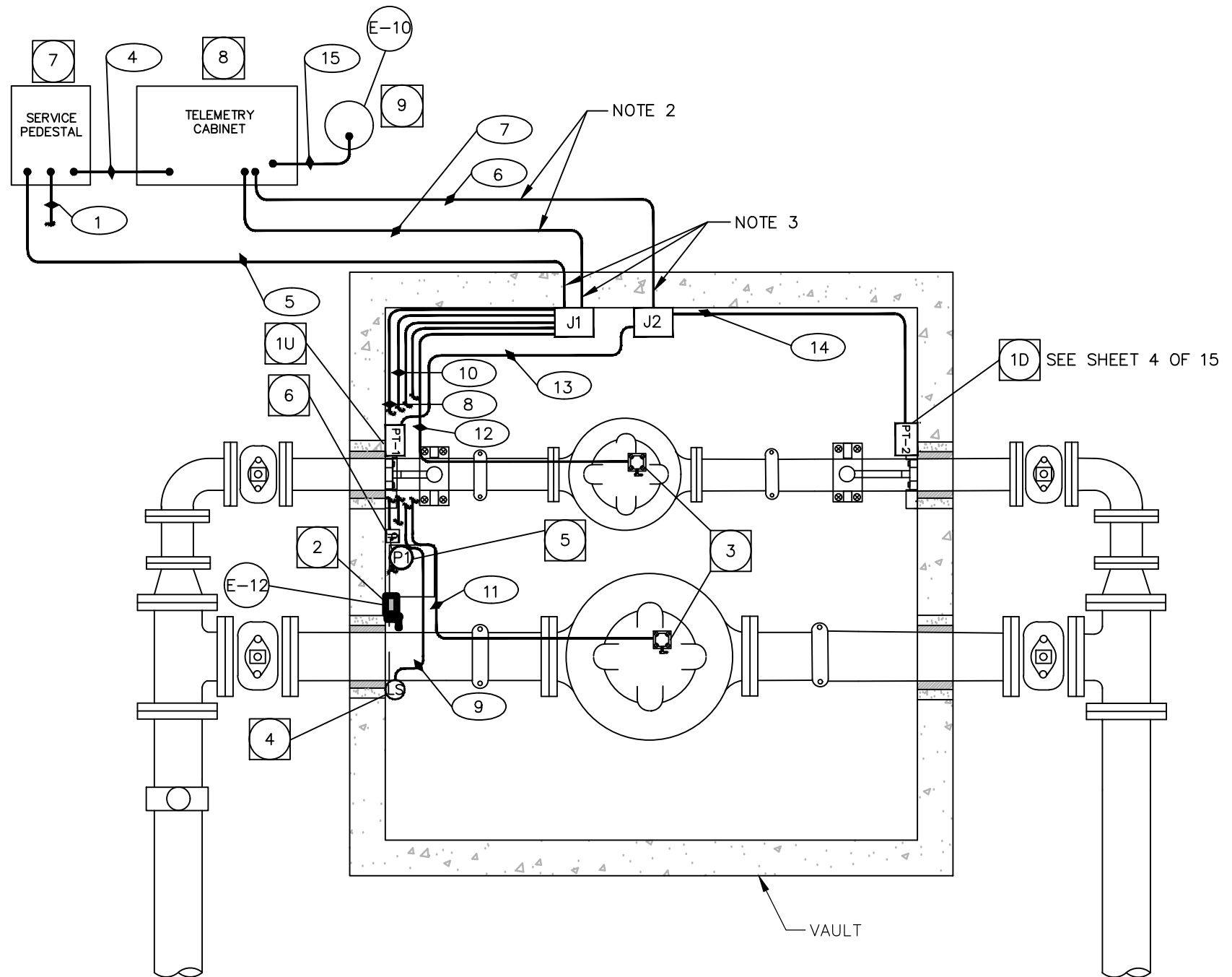
PRESSURE REGULATING STATION ELECTRICAL-CONDUIT PLAN (VAULT #1)
