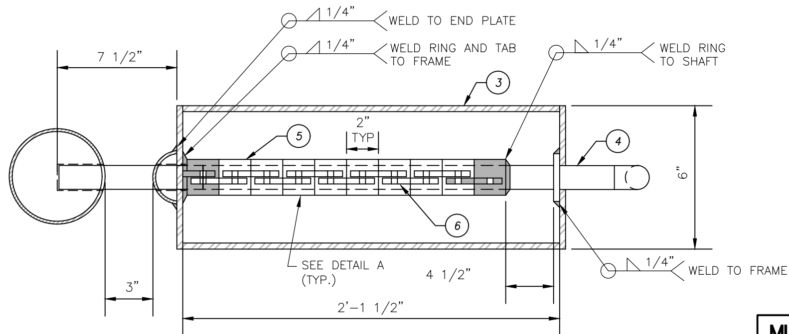
BOTTOM VIEW
