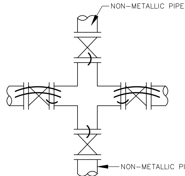
VALVE CROSSING
