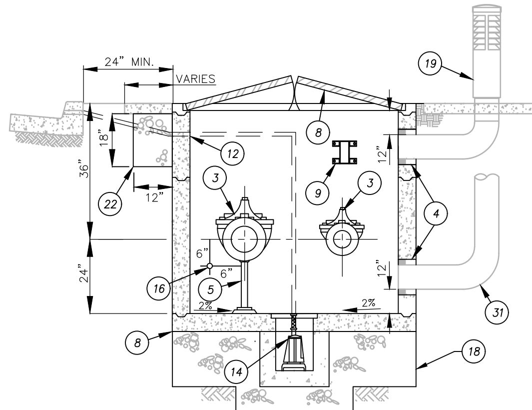
SECTION B-B
