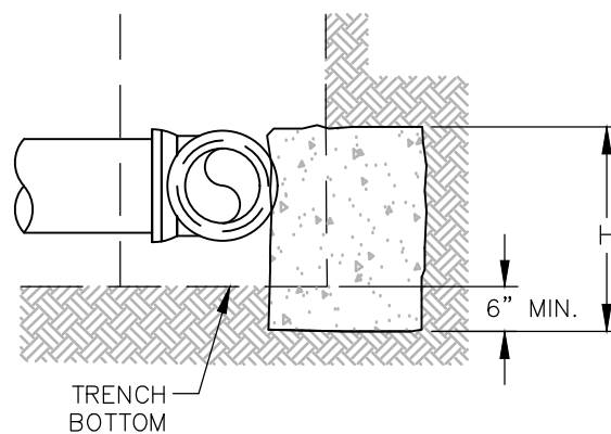
SECTION TEE
