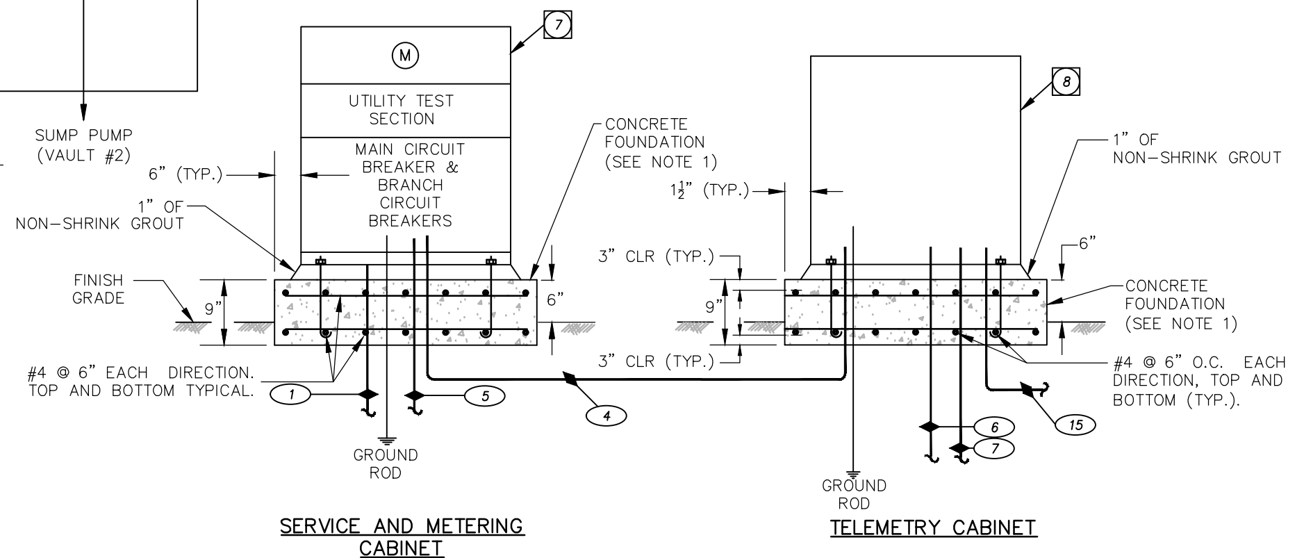
CABINET ELEVATIONS
