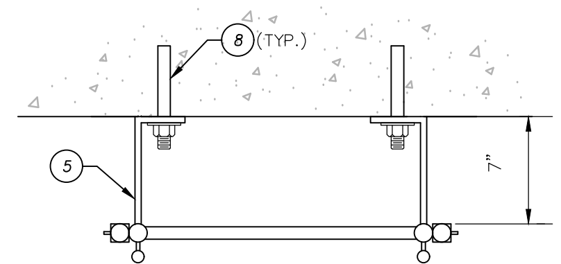
TOP VIEW (DOUBLE HANDRAIL OPTION SHOWN)
