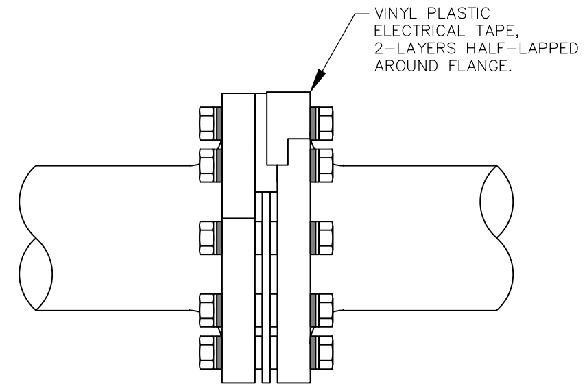
ABOVE GROUND INSULATING FLANGE COATING
