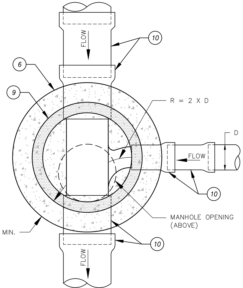
PLAN - MANHOLE BASE
