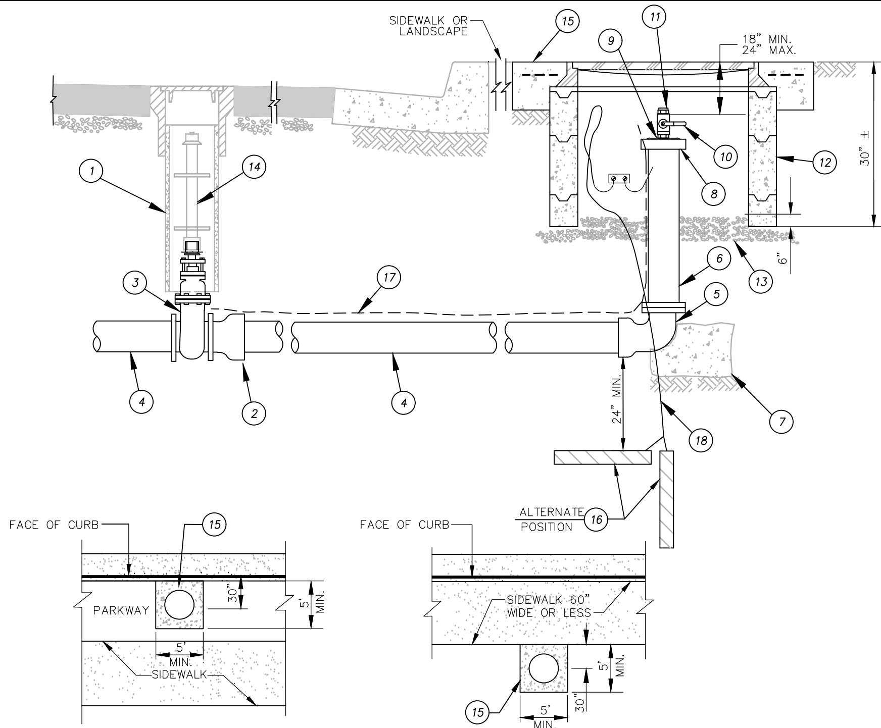
FLUSH-OUT ASSEMBLY LOCATION PLANS
