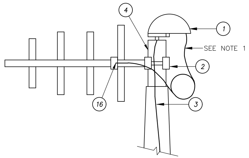
ANTENNA DETAIL
