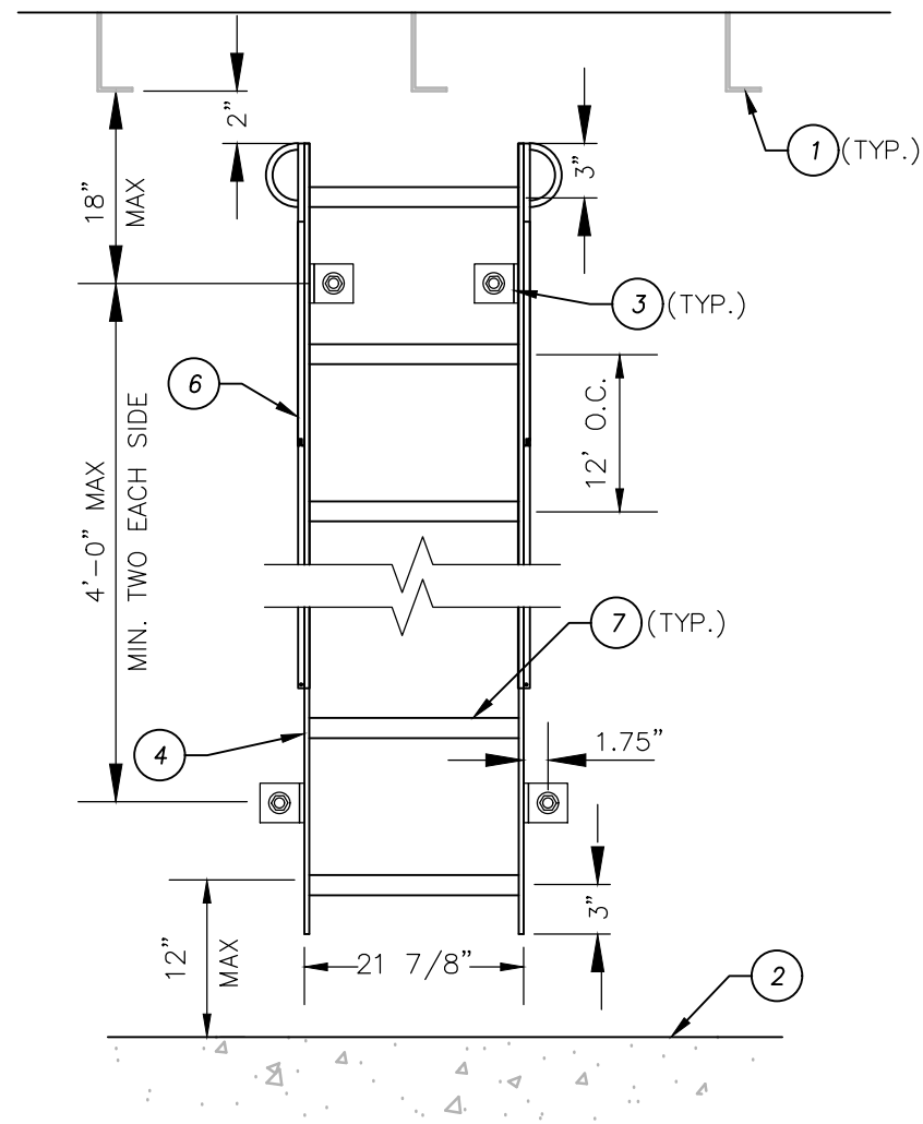
FRONT VIEW DOUBLE HANDRAIL OPTION
