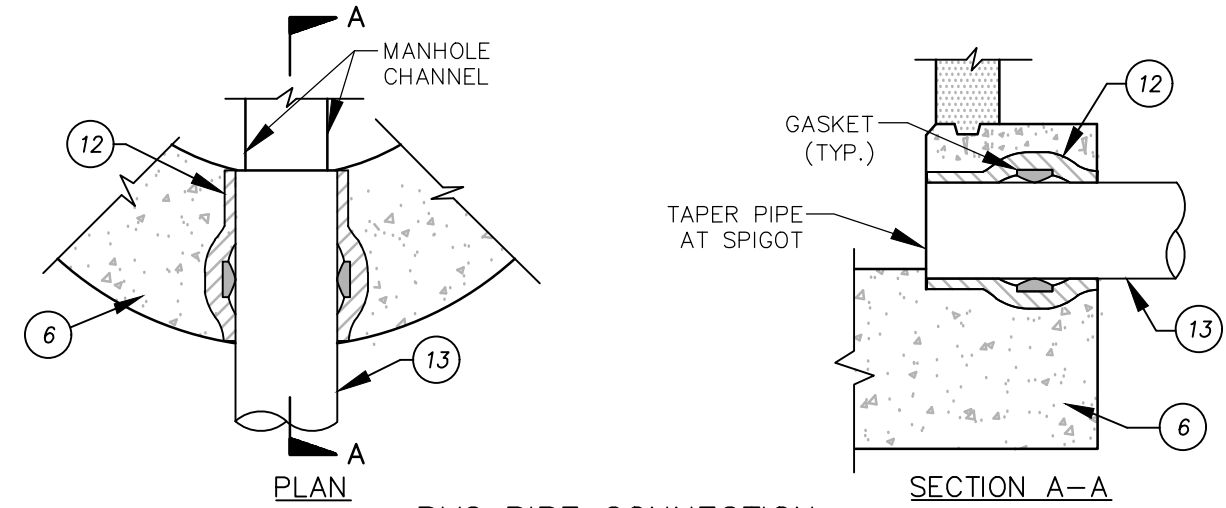
PVC PIPE CONNECTION
