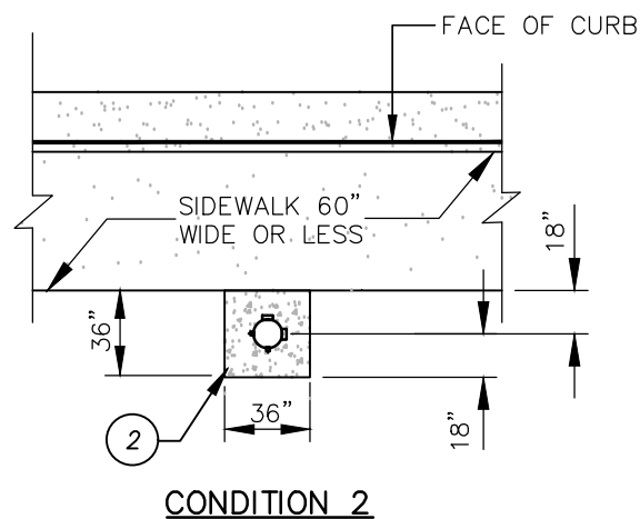
HYDRANT LOCATION PLANS
