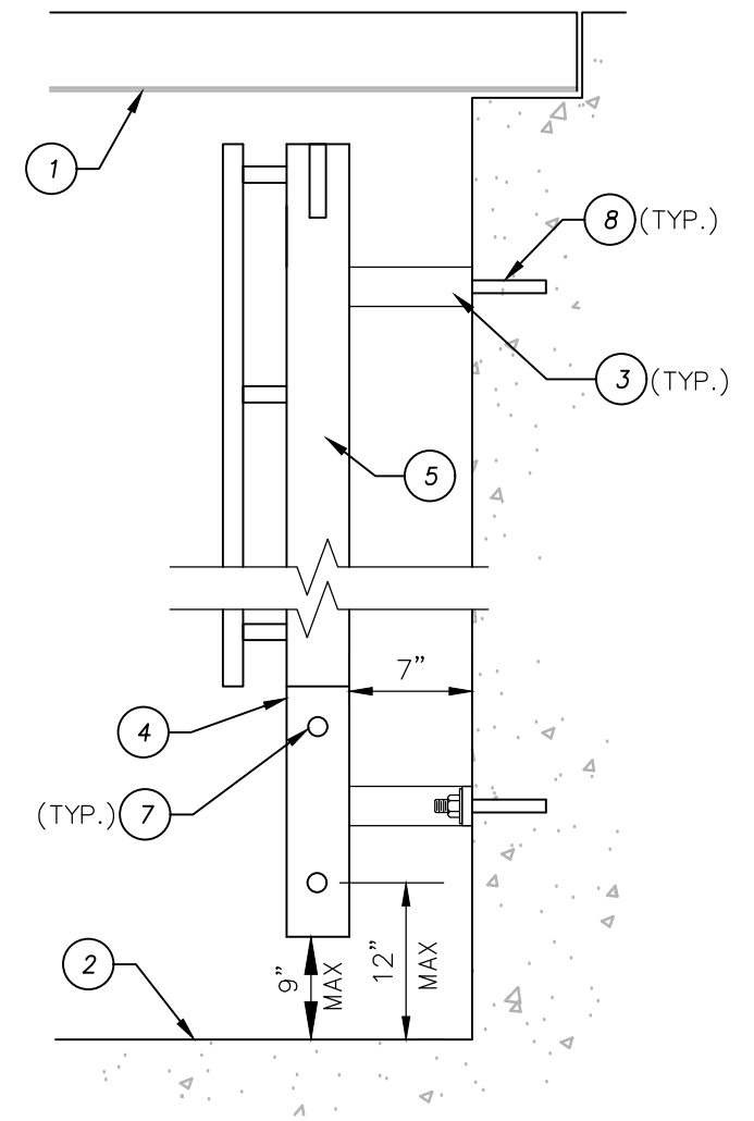
SIDE VIEW (DOUBLE HANDRAIL OPTION SHOWN)
