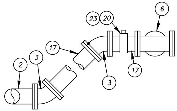
OFFSET PROFILE
